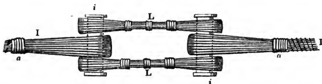
Plan of linking the Cables together.
